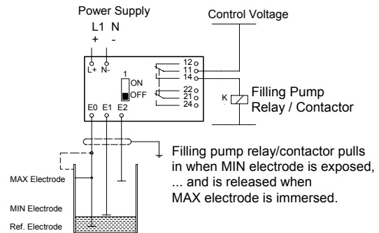
Wiring Diagram 1: Filling the Container
