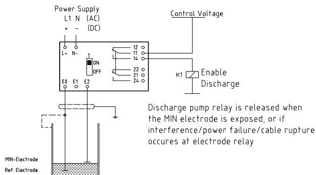
Wiring Diagram 2: Empty Alarm
